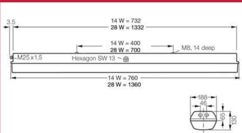
Dimension drawing nLLK 10014/14 / nLLK 10028/28
