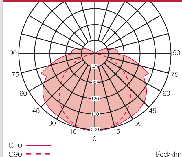
Polar curve nLLK 10014/14 / nLLK 10028/28
