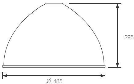
Sand Aluminium Reflector Code : 331057
